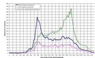
Figure 3: Average weekly 15 minute traffic volumes recorded on each approach to the roundabout
